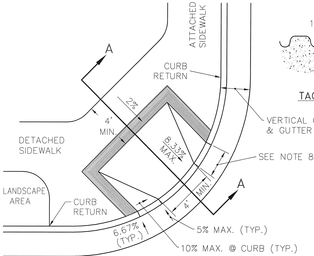
WHEELCHAIR RAMP N.T.S.
