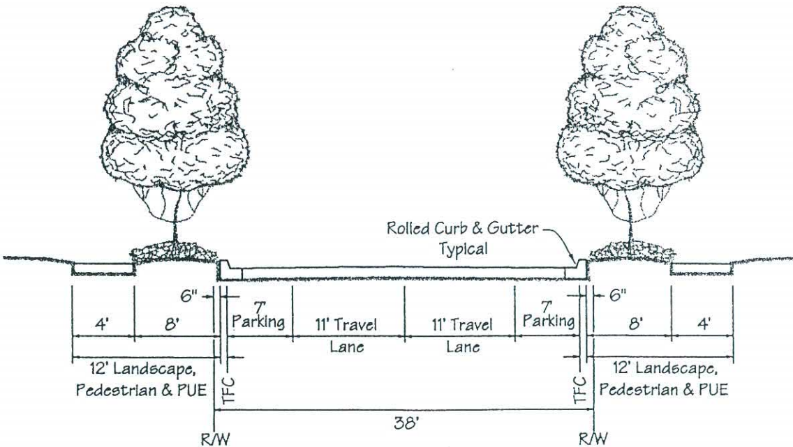
MINOR RESIDENTIAL OVER 500 ADT WITH SEPARATED SIDEWALK
