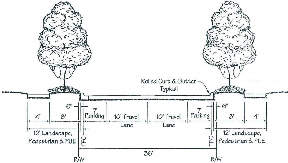
MINOR RESIDENTIAL UNDER 500 ADT WITH SEPARATED SIDEWALK
